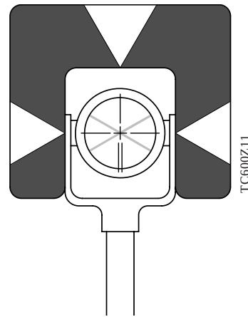
GPH1 single-prism holder with GZT4 target plate
