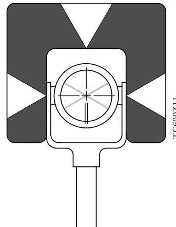
GPH1 prism holder with GZT4 target plate
