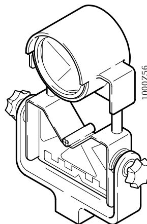
GPH1Z/GRZ3 single-prism holder
